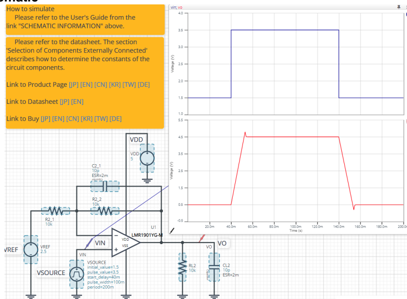
Figure 1. Simulation Schematic
