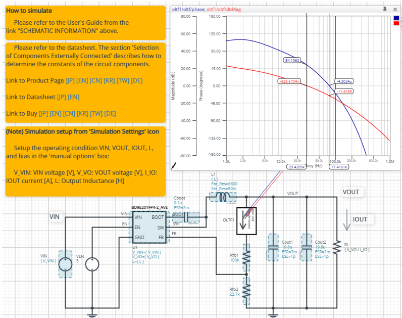
Figure 1. Simulation Circuit
