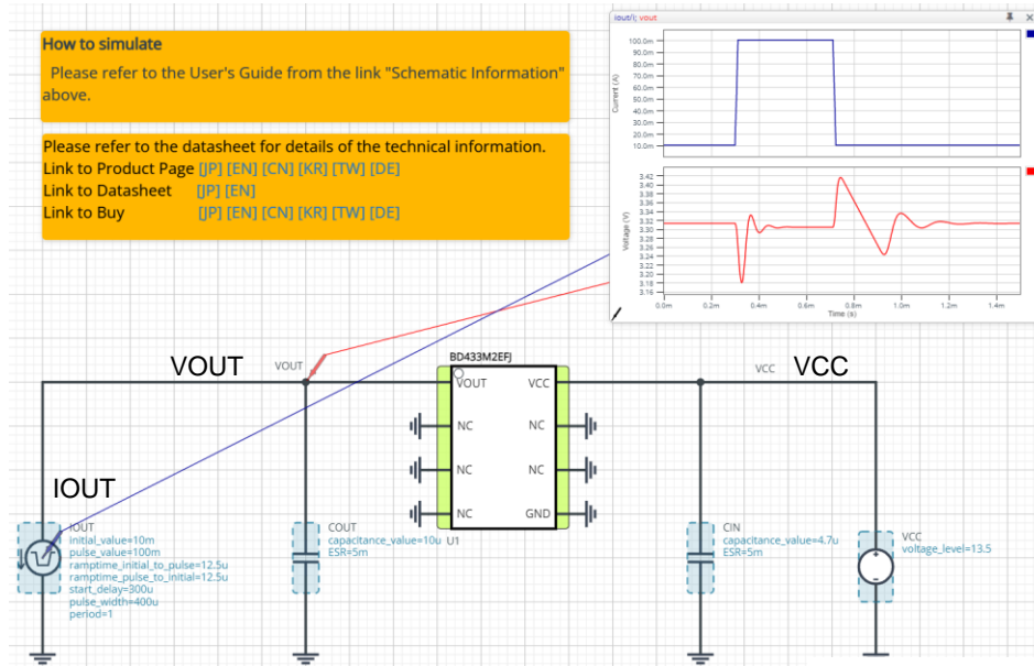
Figure 1. Simulation Schematic
